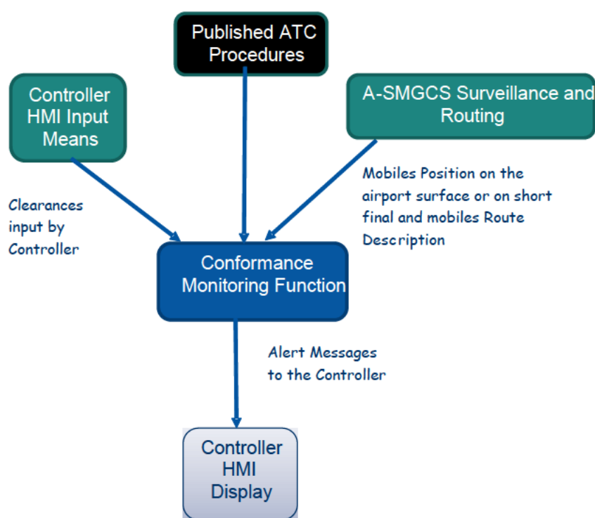
Figure 10 – Conformance monitoring alerts – Ground functional architecture
