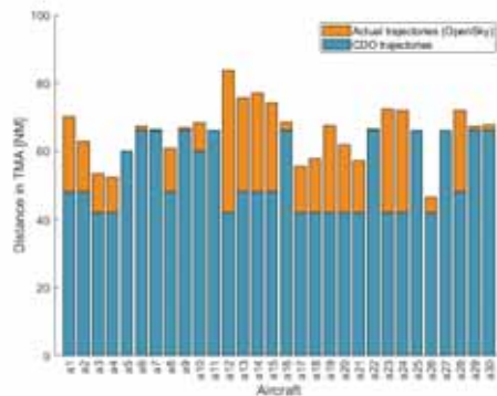
Figure 7. Comparison of the distance flown in the TMA of the actual (orange) vs. optimized CDO-enabled routes (blue) for 30 arrivals within Stockholm TMA on May 16, 2018.
