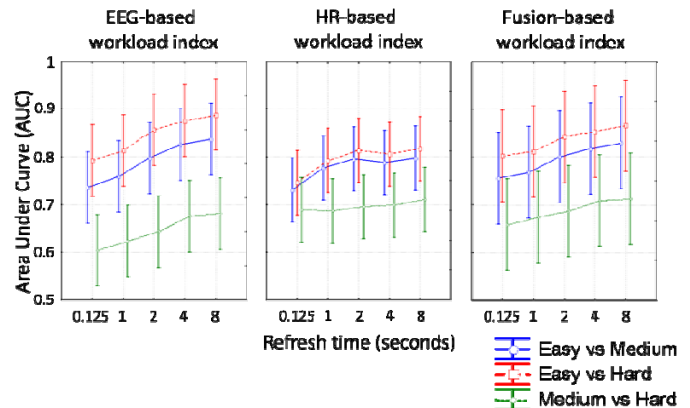
Figure 9. Mean values and related standard errors (CI = .95) of the AUC values achieved using the different classifiers (EEG, HR and Fusion-based) for each refresh time value.
